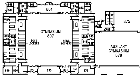
BUILDING 800 GROUND FLOOR PLAN
