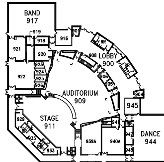
BUILDING 900 GROUND FLOOR PLAN
